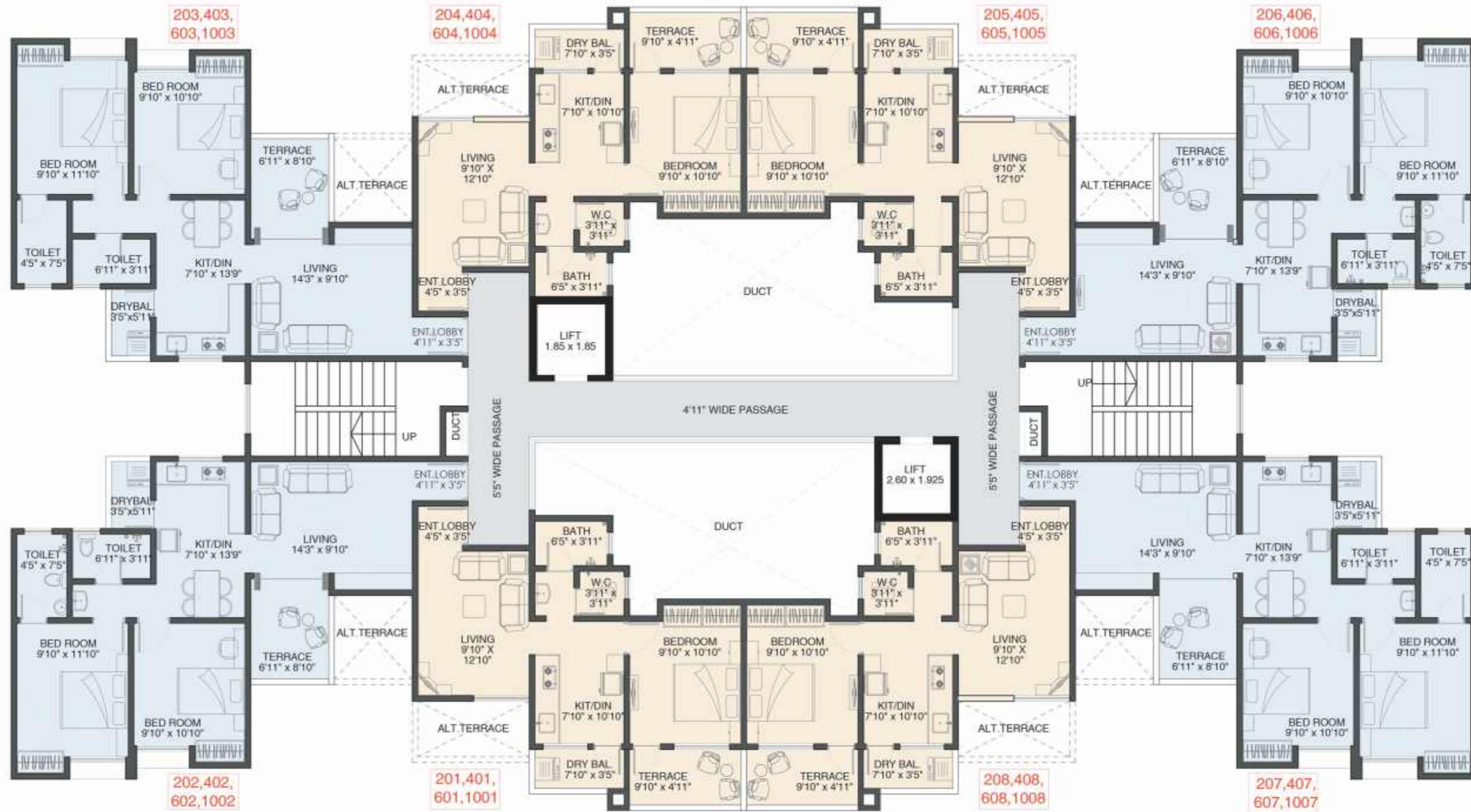
B WING EVEN FLOOR PLAN
