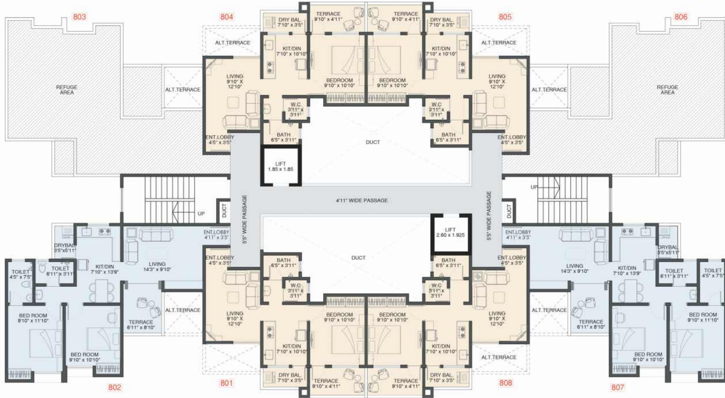
B WING ( 8th FLOOR PLAN )
