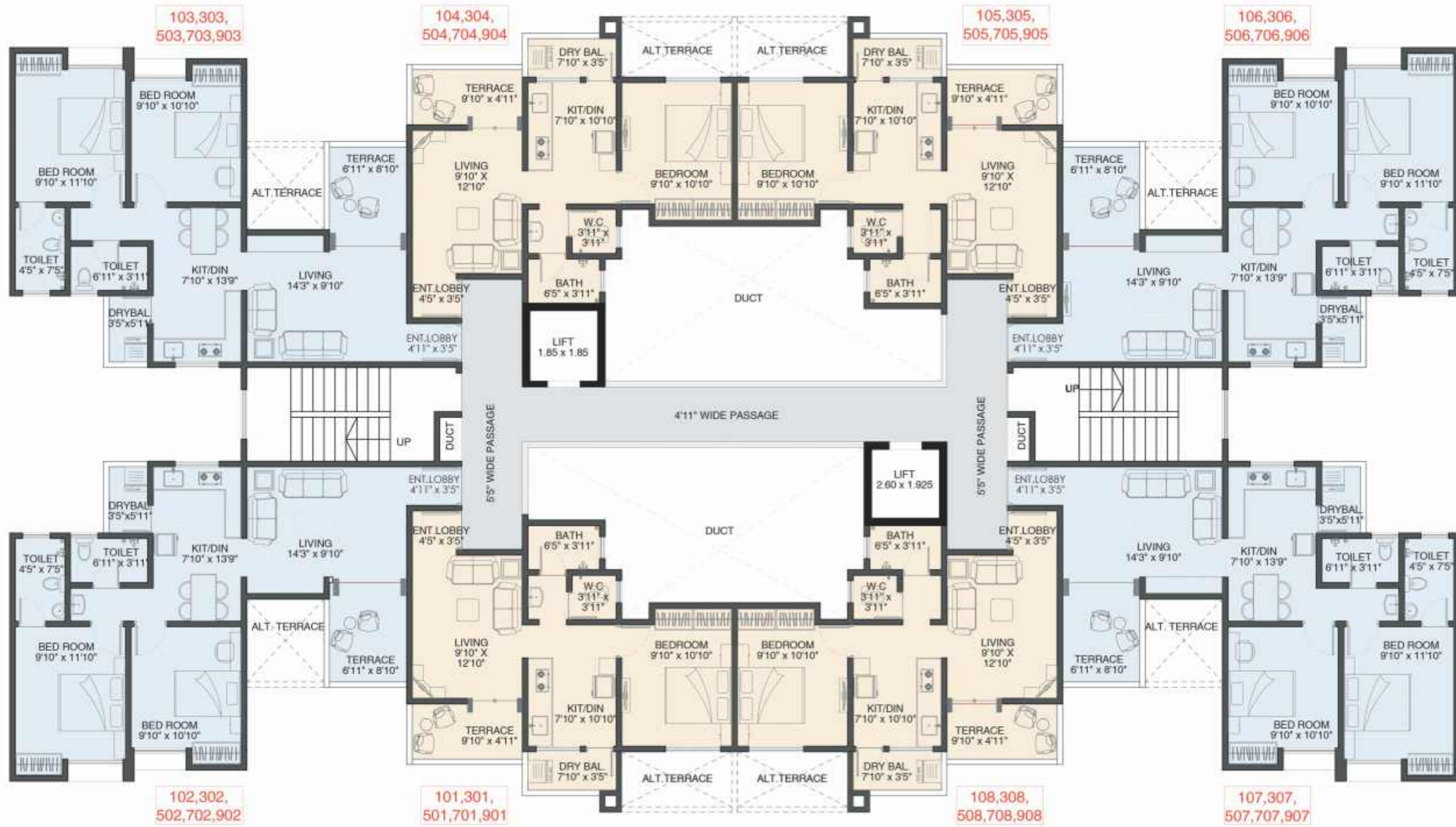
B WING ODD FLOOR PLAN
